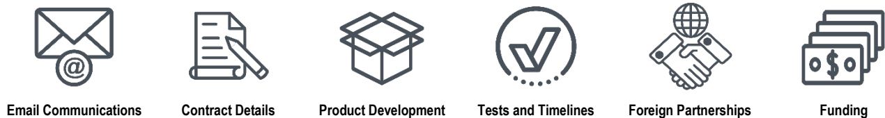
Figure 2. Exfiltrated Information
